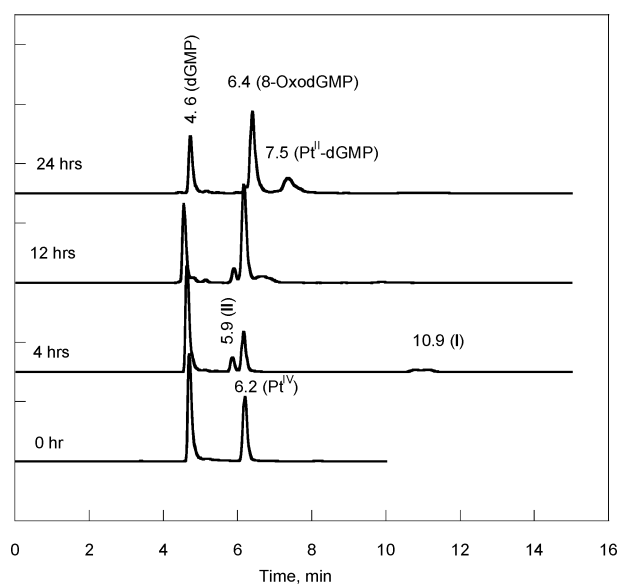
Figure 3. Reversed-phase HPLC chromatograms (DAD, \lambda = 294 nm) of the reaction of 10 mM [\text{Pt}^{\text{IV}}\text{Cl}_4(\text{dach})] with 20 mM dGMP at pH 8.6 ( t = 0 ) and 37 ^\circ\text{C} .
