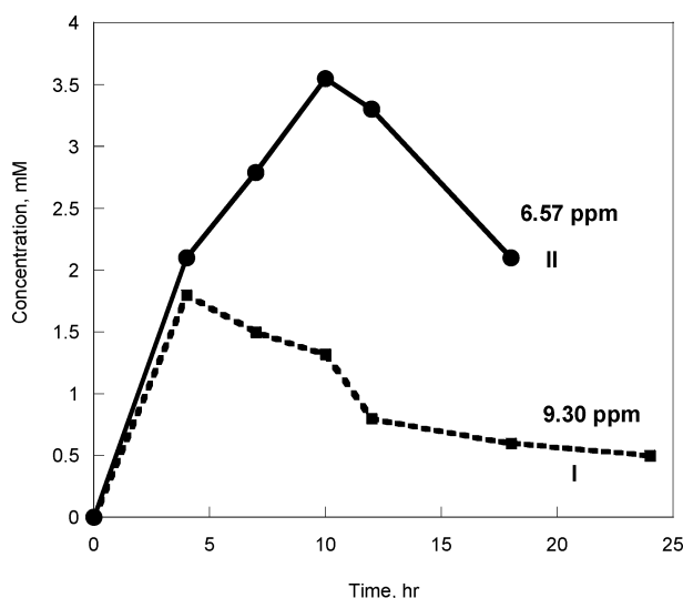
Figure 2. Time-dependent concentrations of I and II generated from the reaction of 10 mM [\text{Pt}^{\text{IV}}\text{Cl}_4(\text{dach})] with 20 mM dGMP at pH 8.6 ( t = 0 ) and 37 ^\circ\text{C} . They were calculated from the ^1\text{H} NMR peaks at 9.30 and 6.57 ppm, respectively.
