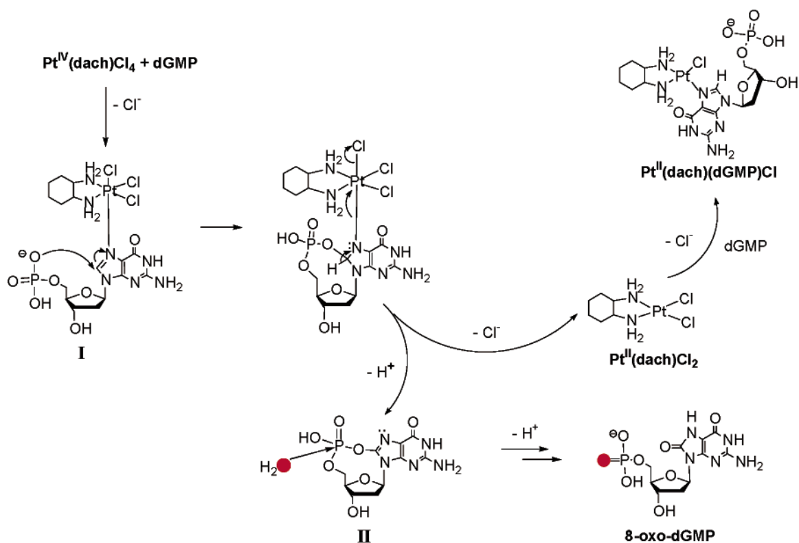
Scheme 1. Proposed Mechanism
